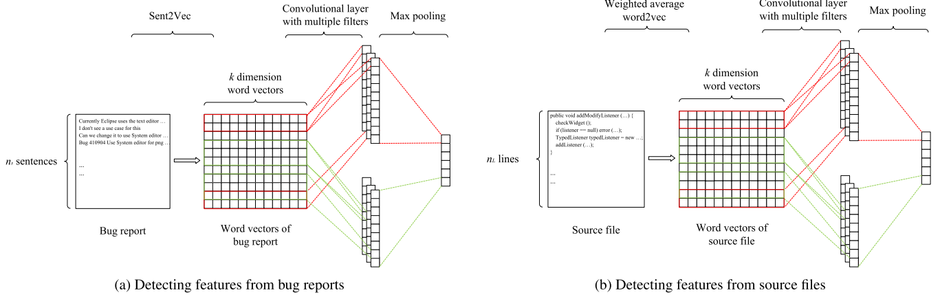
Fig. 7. The architecture of feature detection.
