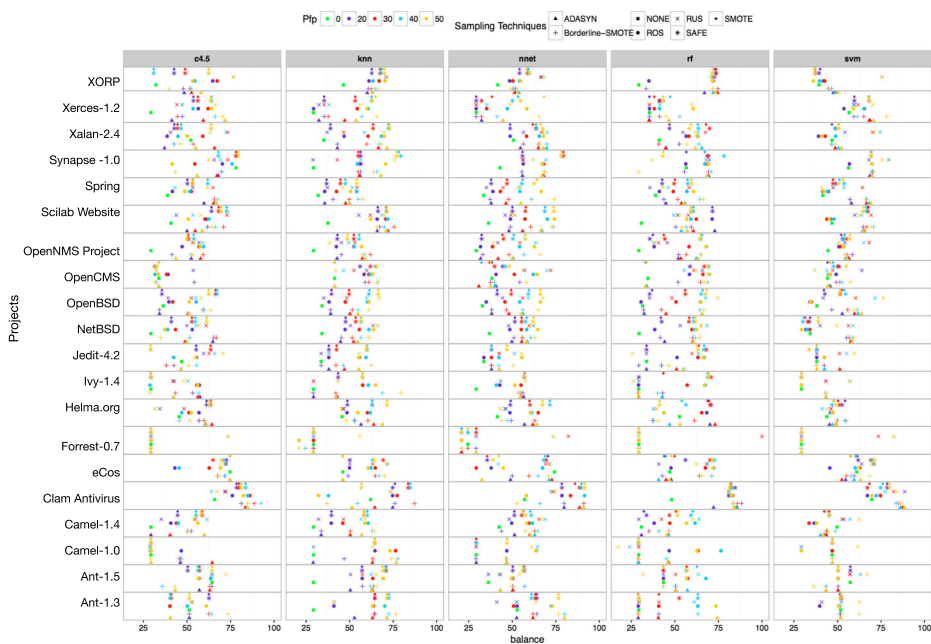
Fig. 13 Performance plot of the sampling approaches per each prediction model for the balance performance measure on 20 imbalanced datasets across different percentage of fault-prone modules ( Pfp ) values
