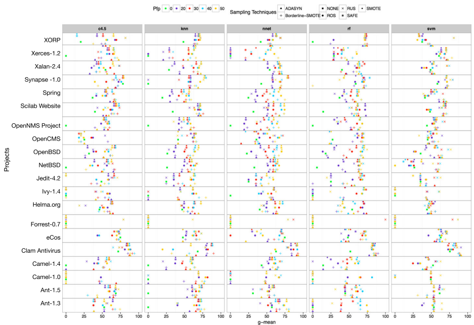
Fig. 12 Performance plot of the sampling approaches per each prediction model for the g -mean performance measure on 20 imbalanced datasets across different percentage of fault-prone modules ( P_{fp} ) values
