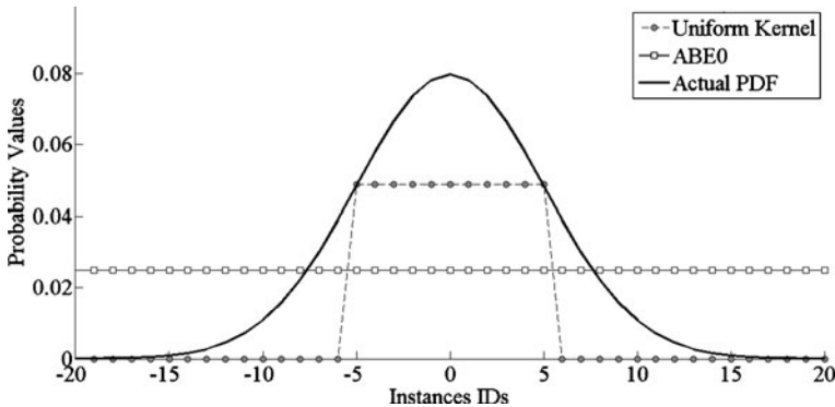
Fig. 2 In the case of ABE0 all instances are given equal probability values, hence equal weights. However, uniform kernel prefers some instances over the others: only a certain portion of the instances are given equal non-zero weights
