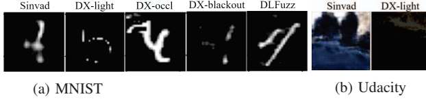
Fig. 2: Invalid test inputs for MNIST and Udcity datasets.
