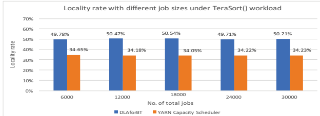
Fig. 2. Locality rate on TeraSort() jobs workload
