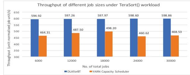
Fig. 3. Throughput on TeraSort() jobs workload
