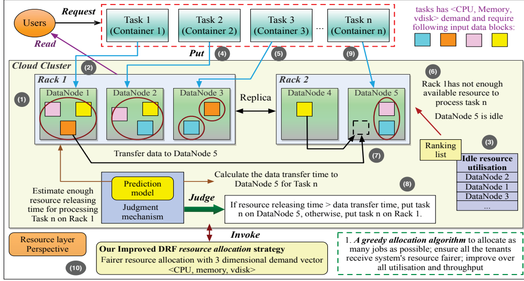
Fig. 1. DLAforBT scheduler architecture: moving computation or moving data
