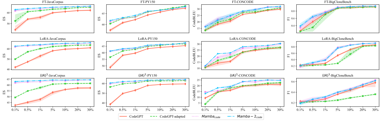
Fig. 3. Evaluation results in the low-resource scenario.
