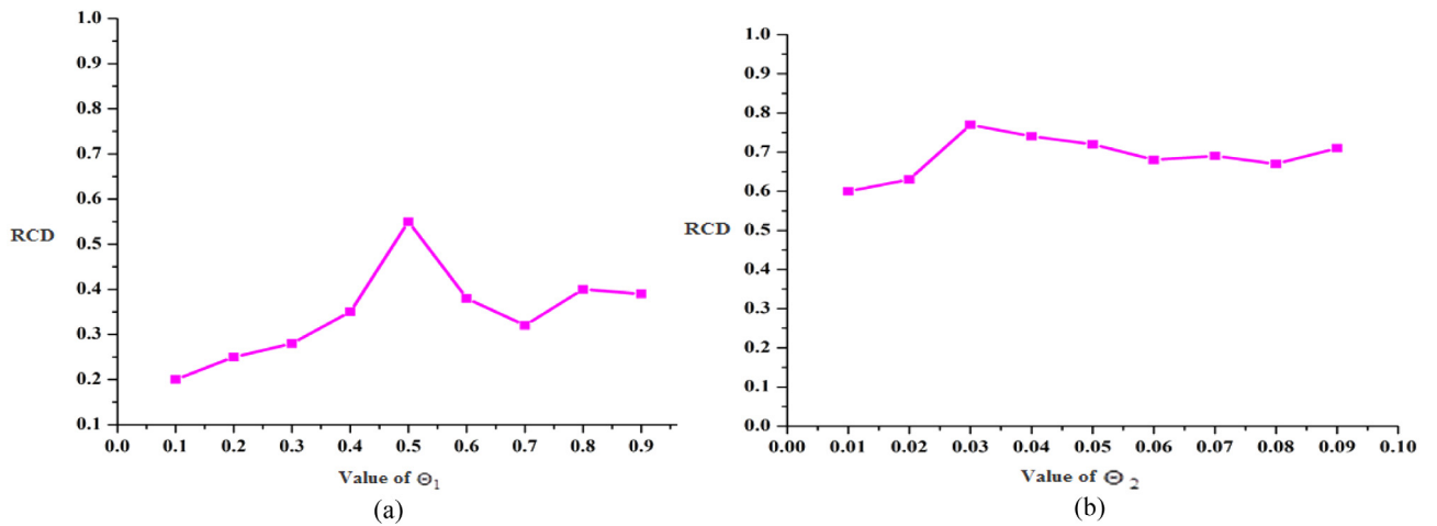
Fig. 12. First Sample of 30 design problems. (a) Mean RCD for first similarity option (Eq. (5)) (b) Mean RCD for second similarity option (Eq. (6)).
