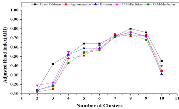
Fig. 10. Evaluation results of unsupervised learners with their Best weighting methods on Security design problems.
