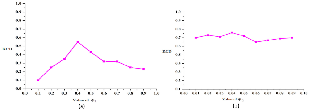
Fig. 11. First Sample of 9 design problems. (a) Mean RCD for second similarity option (Eq. (5)) (b) Mean RCD for third similarity option (Eq. (6)).
