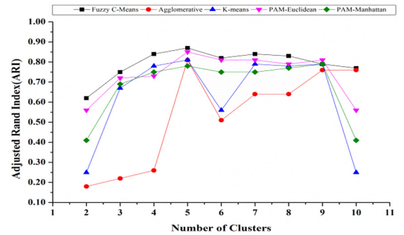
Fig. 9. Evaluation results of unsupervised learners with their best weighting methods on Douglass design problems.
