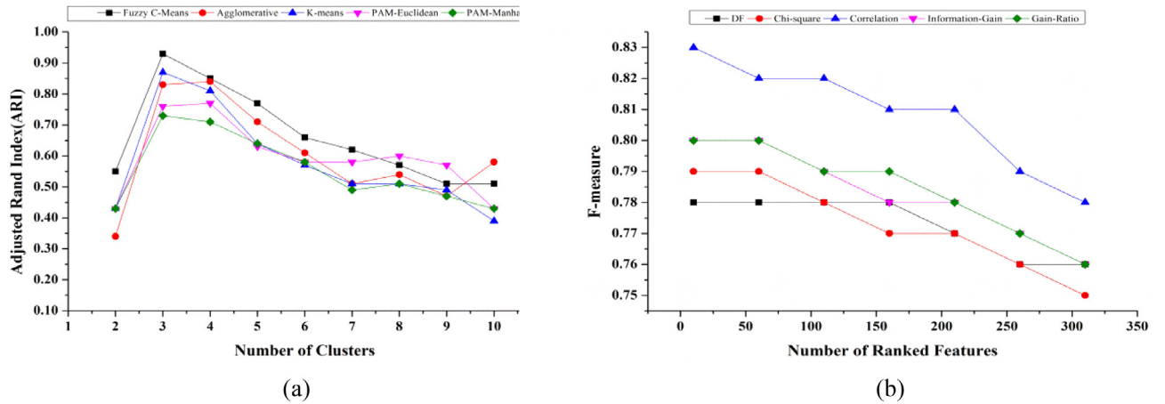
Fig. 5. Evaluation results on GoF patterns. (a) Unsupervised learners with their best weighting method (b) Best unsupervised learner (Fuzzy c-means) with N rank features.
