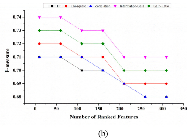
Fig. 6. Evaluation results on Douglass patterns. (a) Unsupervised learners with their best weighting method (b) Best unsupervised learner (PAM-Euclidean) with N rank features.
