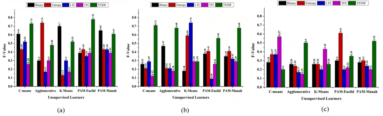
Fig. 4. Best weighting methods for unsupervised learners (a) GoF patterns (b) Douglass patterns (c) Security patterns collection.
