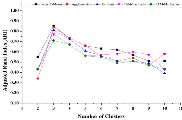
Fig. 8. Evaluation results of unsupervised learners (with their best weighting methods) on GoF design problems and sample of 31 design problems.
