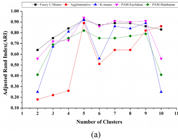
Fig. 6. Evaluation results on Douglass patterns. (a) Unsupervised learners with their best weighting method (b) Best unsupervised learner (PAM-Euclidean) with N rank features.
