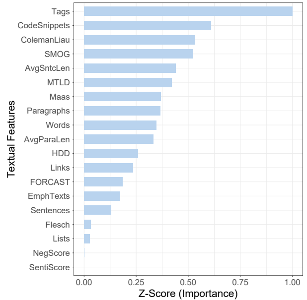
Fig. 3. Rank Features by Importance
